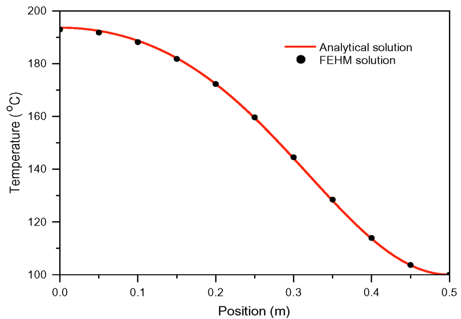
Figure 7. Comparison of FEHM and analytical solutions for 2-D heat conduction at time t = 2.16 \times 10^4 seconds.
