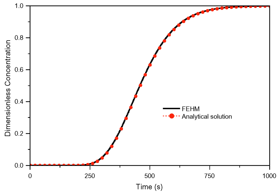
Figure 40. Comparison of FEHM results with the analytical solution for a mobile water phase.
