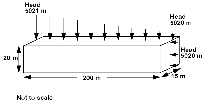
Figure 27. Model domain and flow boundary conditions for the streamline particle tracking reverse tracking model test problems.
