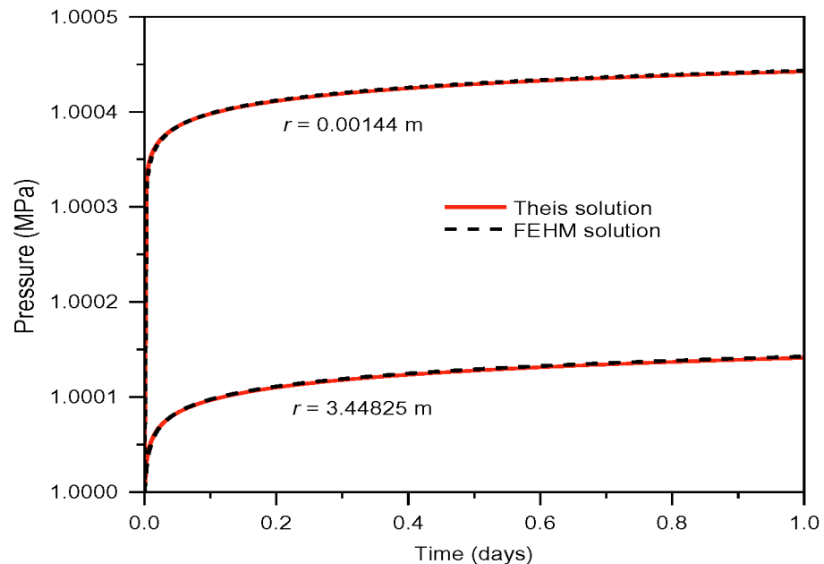
Figure 13. Comparison of FEHM and Theis solutions for pressure vs. time at r = 0.00144 m and r = 3.44825 m from the wellbore.
