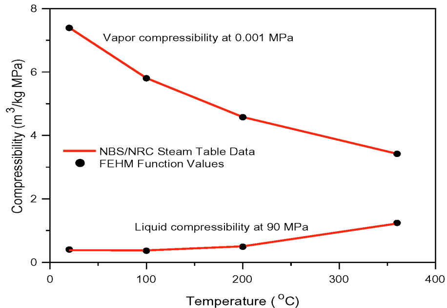
Figure 3. Comparison of FEHM compressibilities to National Bureau of Standards Steam Table Data.
