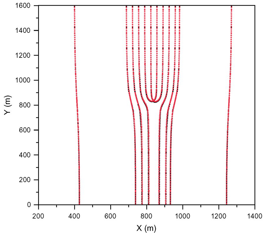
Figure 53. Comparison of particle tracks for the particle capture model using a coarse and fine grid.
