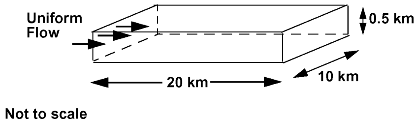
Figure 26. Model domain and flow boundary conditions for the streamline particle tracking standard dispersion model test problems.
