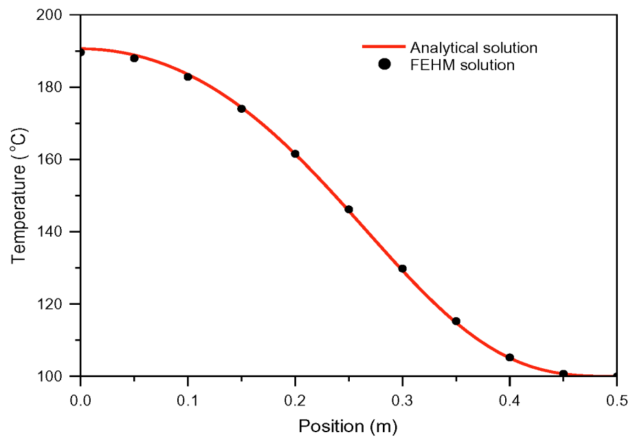
Figure 9. Comparison of FEHM and analytical solutions for 3-D heat conduction at time t = 2.16 \times 10^4 seconds.
