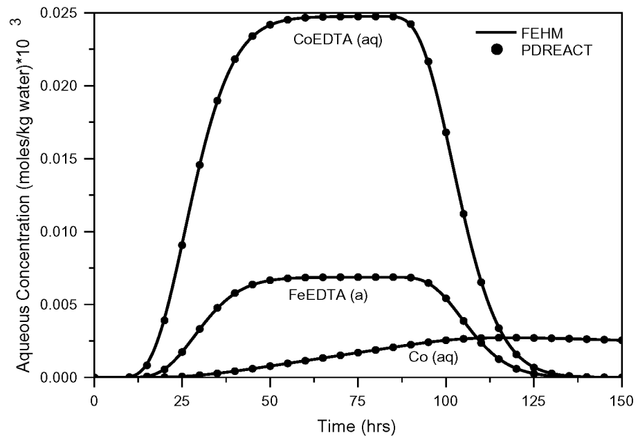
Figure 43. Comparison of FEHM and PDREACT for the breakthrough curves of aqueous species.
